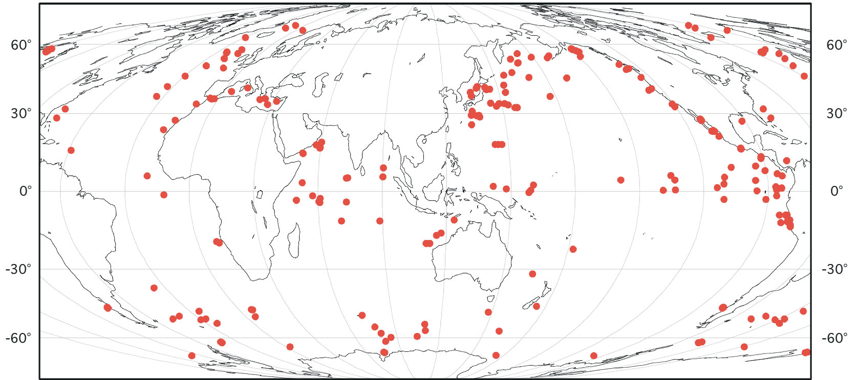
Pleistocene Rad MRC Samples
