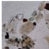
Vitric 17
