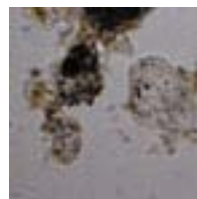
Quartz 7
