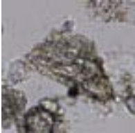
Metamorphic 1
