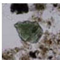
Other dense 1
