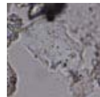
Quartz 5
