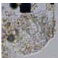
Carbonate 1
