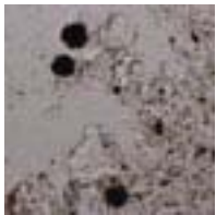
Pyrite 2
