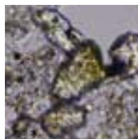
Epidote group 3
