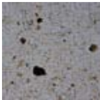
Zeolite 2
