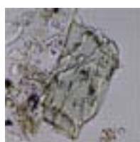
Other dense 2
