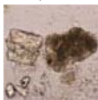
Epidote group 7
