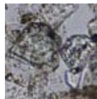
Epidote group 4
