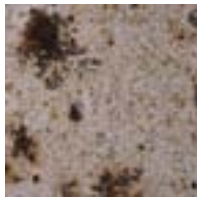
Zeolite 3
