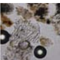
Microlitic 8
