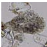
Carbonate 3
