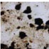
Other sulfides 3
