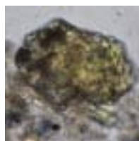
Epidote group 8
