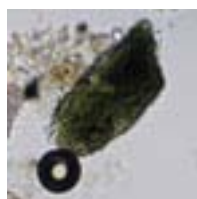
Amphibole 2
