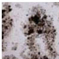
Other sulfides 2
