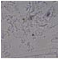
Vitric 1
