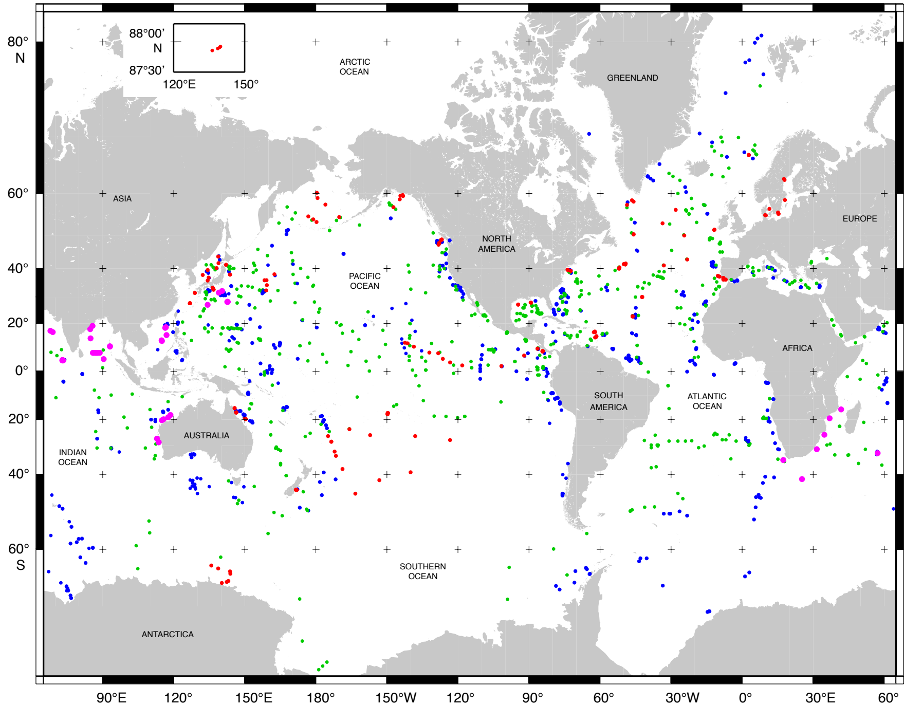
DSDP Legs 1–96 (●), ODP Legs 100–210 (●), IODP Expeditions 301–348 (●), IODP Expeditions 349–361 (●)
